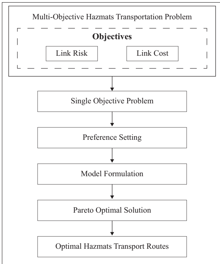
Figure 1: Conceptual Framework
