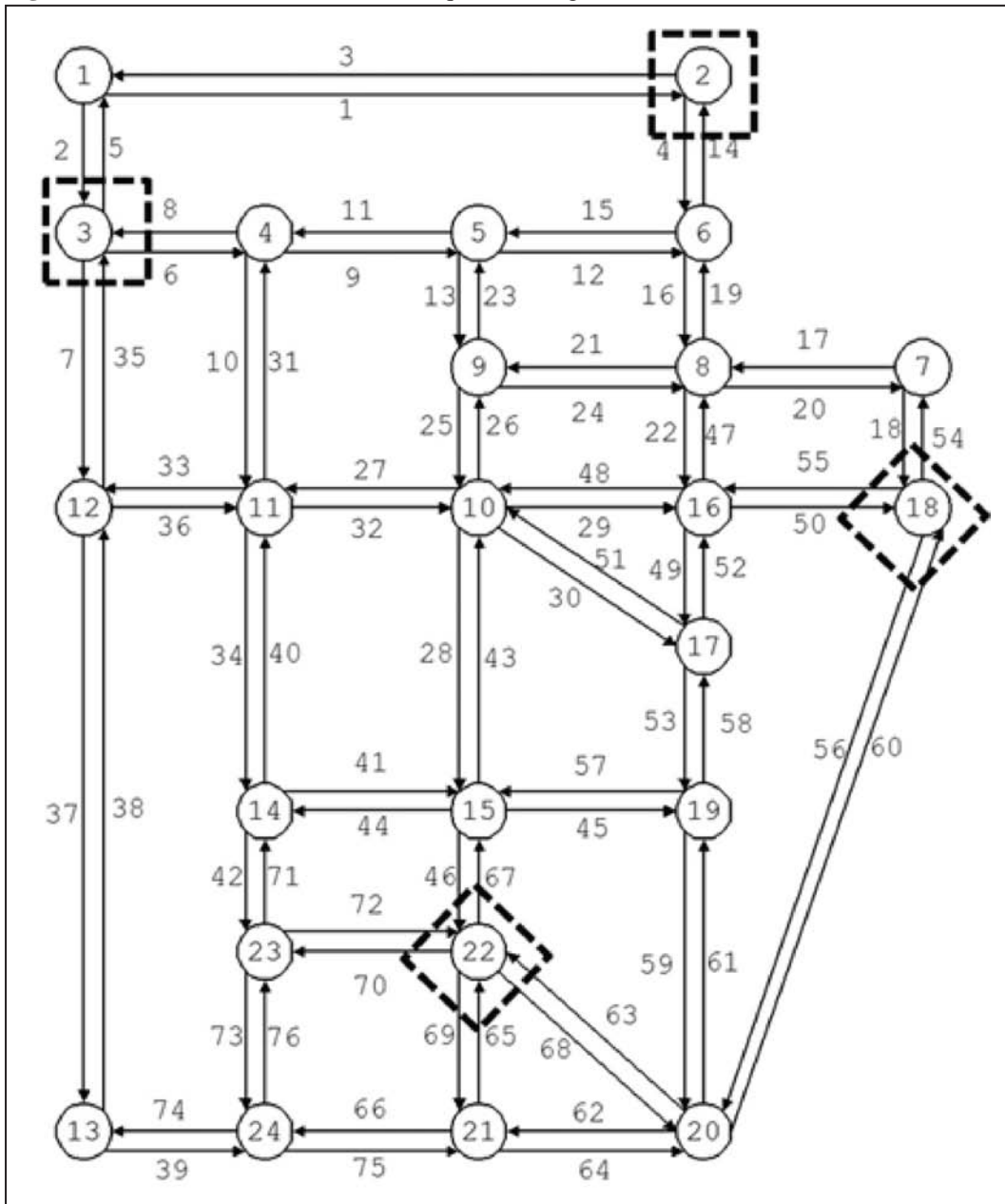
Figure 2: Sioux Falls Network (Dashed Squares = Origins, Dashed Diamonds = Destinations)
